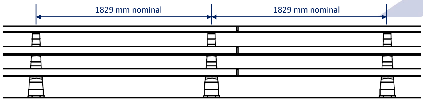
FRONT VIEW
