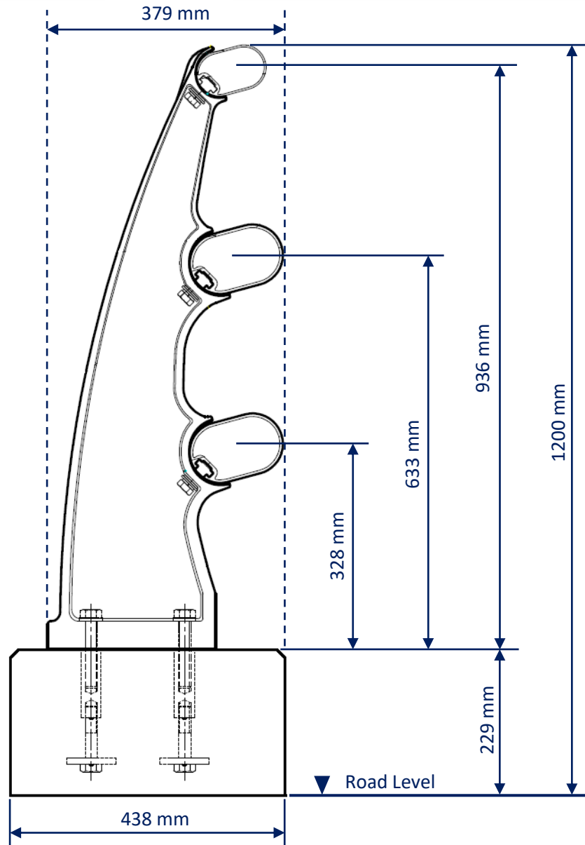
SIDE ELEVATION
